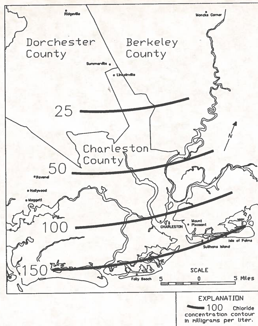
Figure 2. Generalized chloride concentration in deep wells near Charleston, S.C.
