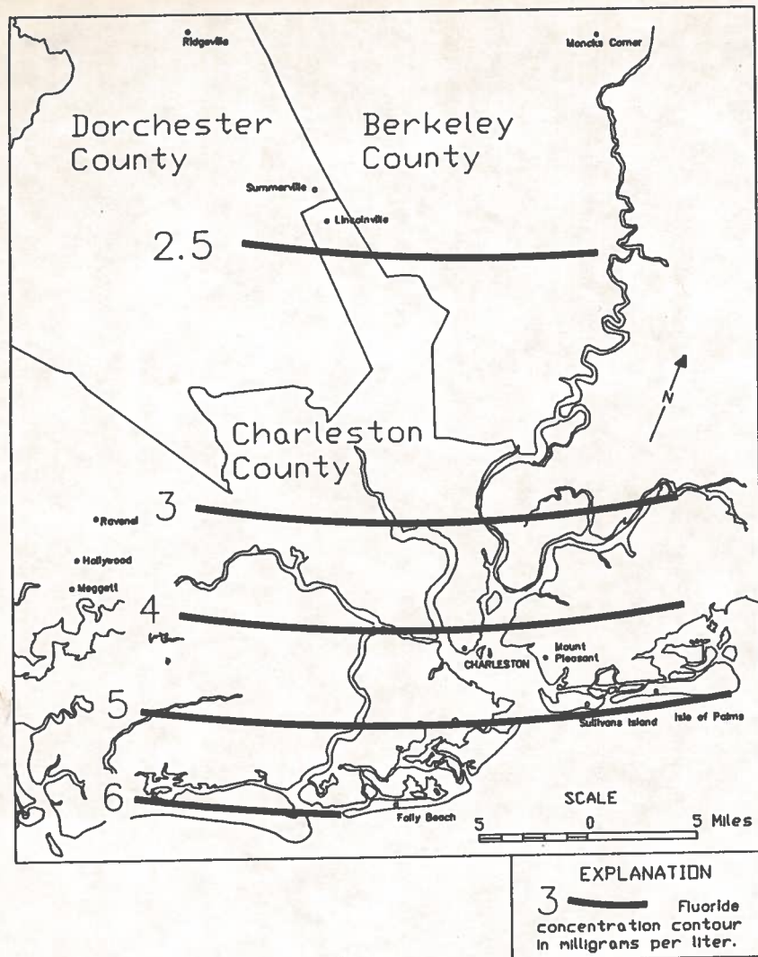
Figure 1. Generalized fluoride concentration in deep wells near Charleston, S.C.
