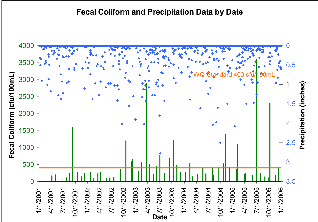
Figure 3. Precipitation and FC Data by Date
