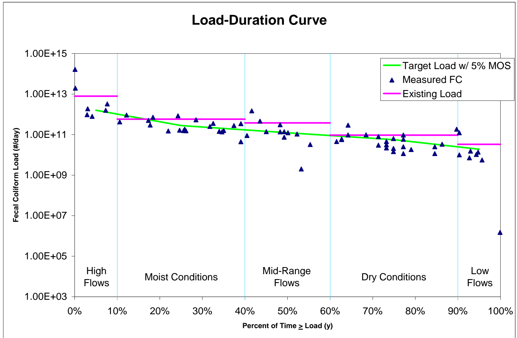
Figure 5. Load Duration Curve for Grannies Quarter Creek Station CW-237
